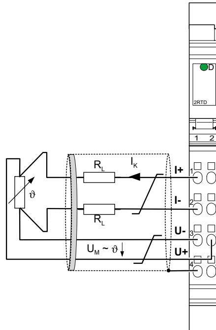
Figure 12 Connection of resistance thermometers in 4-wire technology
